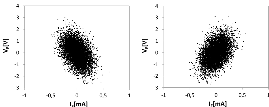
Fig. 2. Scatter plot for cases LH (left) and HL(right) using noise with normal distribution if the Eq. (6) is not satisfied. R_L=1\text{ k}\Omega , R_H=10\text{ k}\Omega , \sigma_{VH}/\sigma_{VL}=1,5 .
