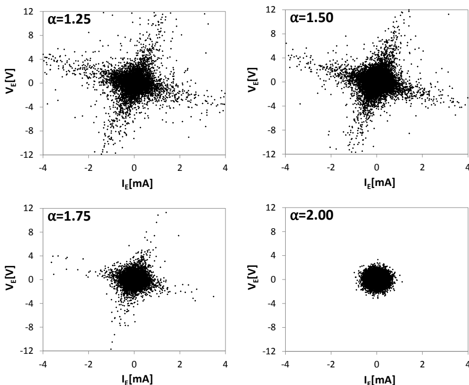
Fig. 3 b. Scatter plot for case HL using distributions with different values of \alpha . Note that \alpha = 1 and \alpha = 2 correspond to Cauchy and normal distribution, respectively. R_L=1 k \Omega , R_H=10 k \Omega , w_{VH}/w_{VL} = \sqrt{R_H/R_L} .
