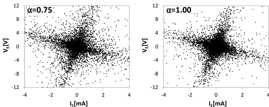
Fig. 3 a. Scatter plot for case HL using distributions with different values of \alpha . Note that \alpha = 1 and \alpha = 2 correspond to Cauchy and normal distribution, respectively. R_L=1\text{ k}\Omega , R_H=10\text{ k}\Omega , w_{VH}/w_{VL} = \sqrt{R_H/R_L} .
