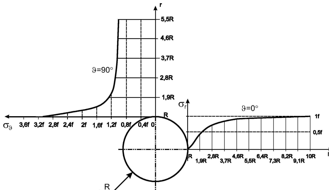
Fig.12.9. Tangential stresses in the plate for \vartheta = 90^\circ and radial stresses for \vartheta = 0^\circ obtained by the finite element solution.
