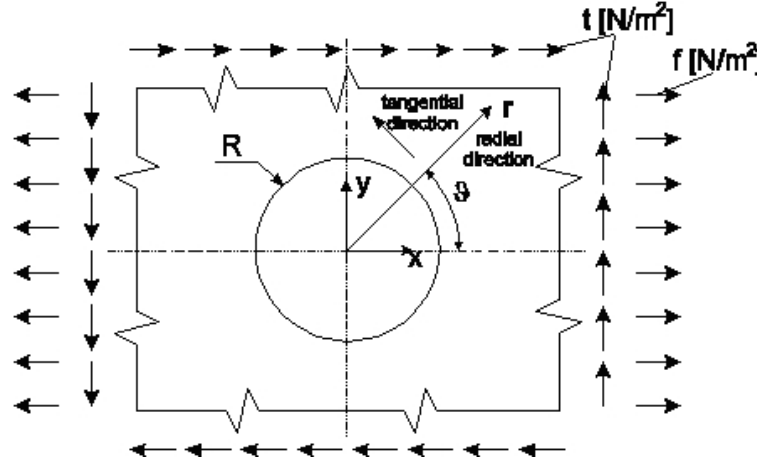
Fig.12.1. Plate with central hole subjected to normal load in direction x and tangential load along the boundaries.
