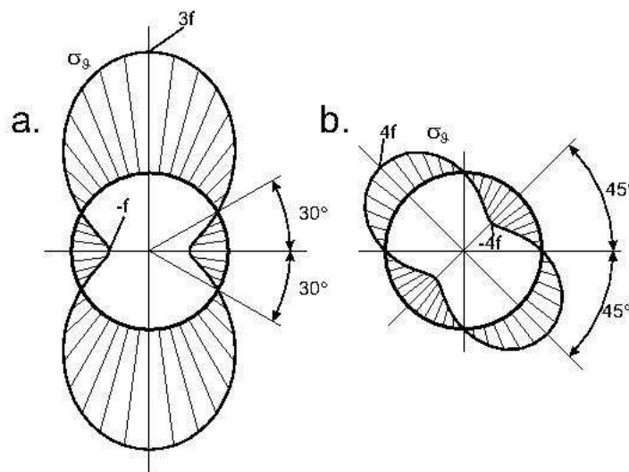
Fig.12.3. Tangential stresses in a plate with circular hole subjected to uniaxial tension in direction x (a) and tangential load along the boundaries (b).
