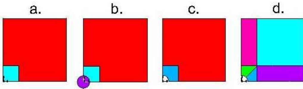
Fig.12.5. Preparation of the geometrical model of a plate with central hole.
