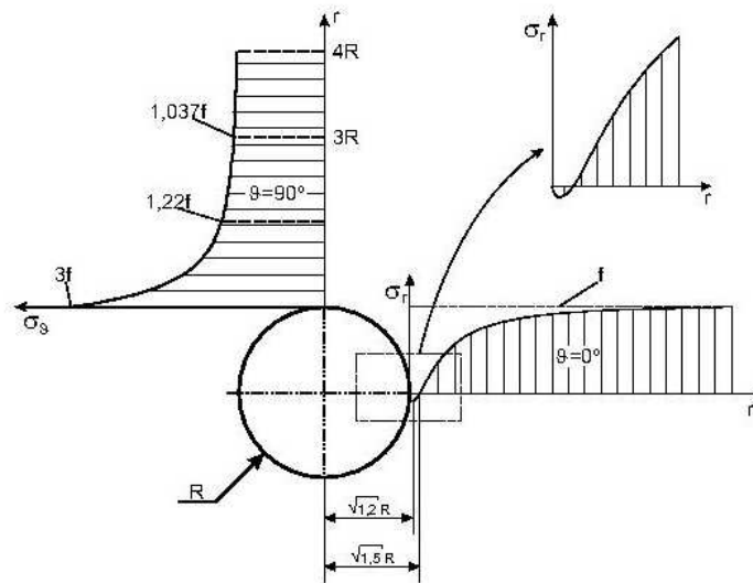
Fig.12.2. Tangential stresses if \vartheta = 90^\circ and radial stresses if \vartheta = 0^\circ in a plate with central hole.
