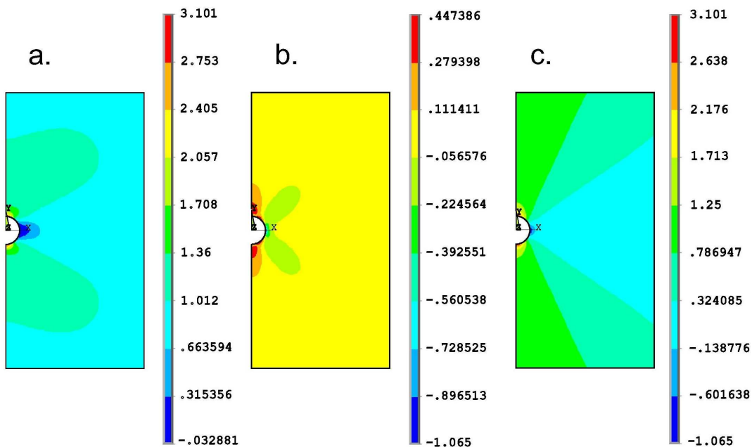
Fig.12.8. Stresses in the finite element model of the plate with hole in [MPa], \sigma_x (a) and \sigma_y (b) in the x-y coordinate system and \sigma_\theta (c) in cylindrical coordinate system.
