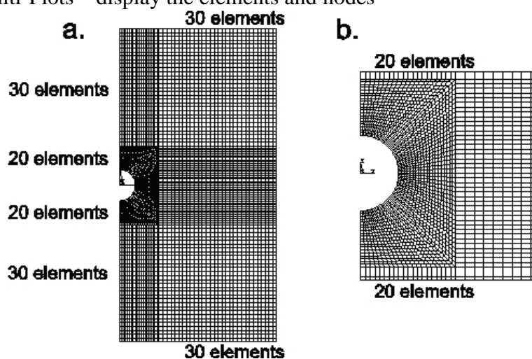
Fig.12.6. Details of the finite element model of the plate with central hole.
