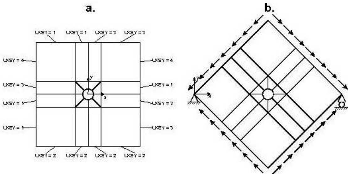
Fig.12.7. Definition of the LKEY parameter for the boundary lines of finite element model of the plate with central hole (a), definition of the boundary conditions by rotating the model (b).
