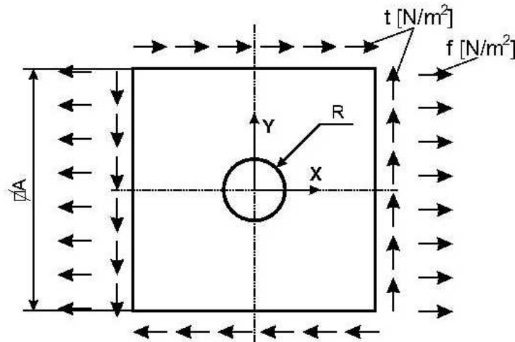
Fig.12.4. Finite dimension plate with central hole subjected to uniaxial tension and tangential load.
