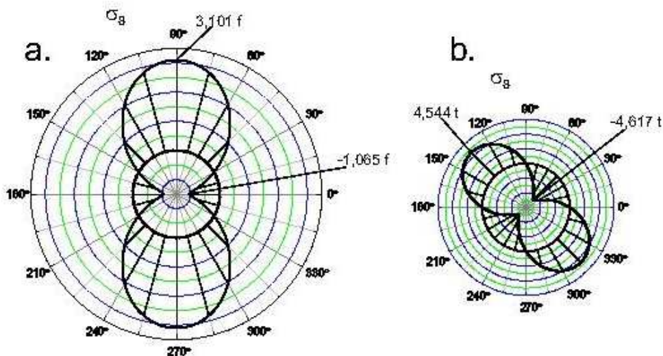
Fig.12.10. Tangential stresses along the hole of the plate with central hole under uniaxial tension in x (a) and tangential load (b) in accordance with the finite element solution.
